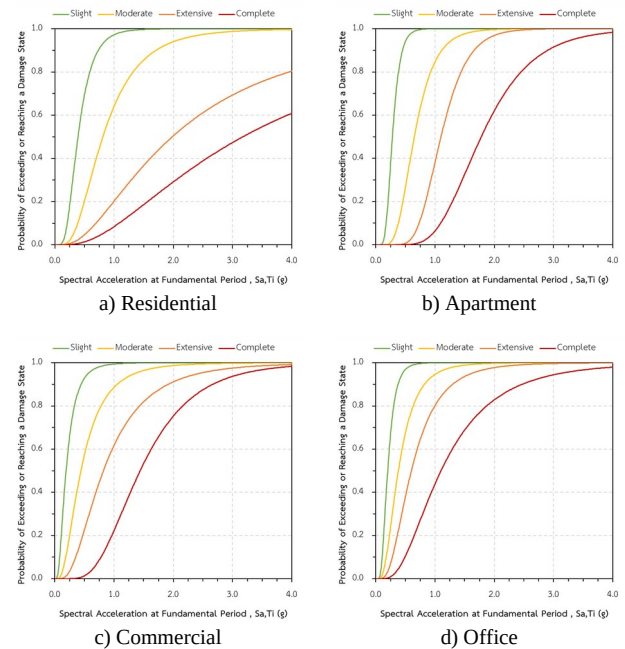
Figure 1. Fragility functions
